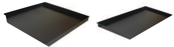
RFU08 Large Vac Form / 1185 w x 940 d x 250 h RFU09 Small Vac Form / 1185 w x 500 d x 250 h
